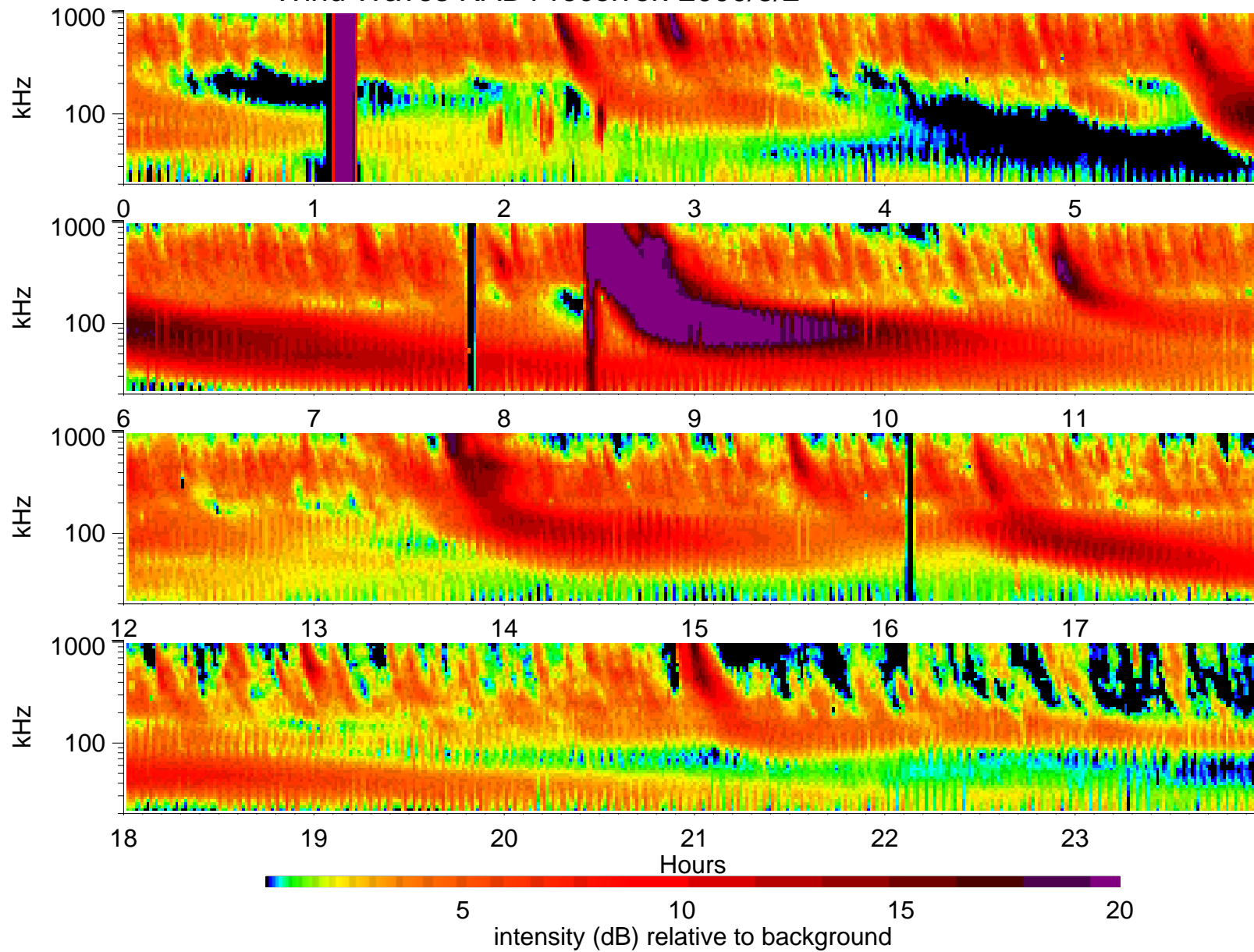
Wind Waves RAD1 receiver: 2000/3/2
