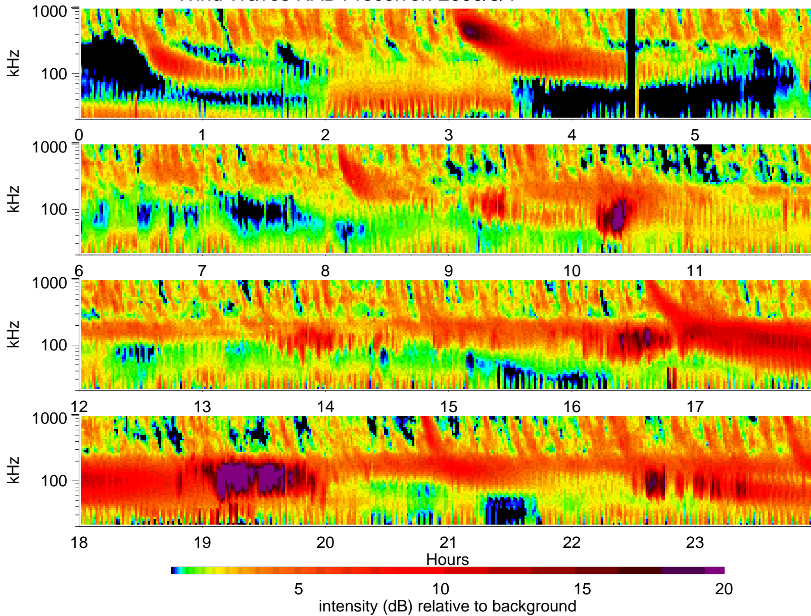
Wind Waves RAD1 receiver: 2000/3/1
