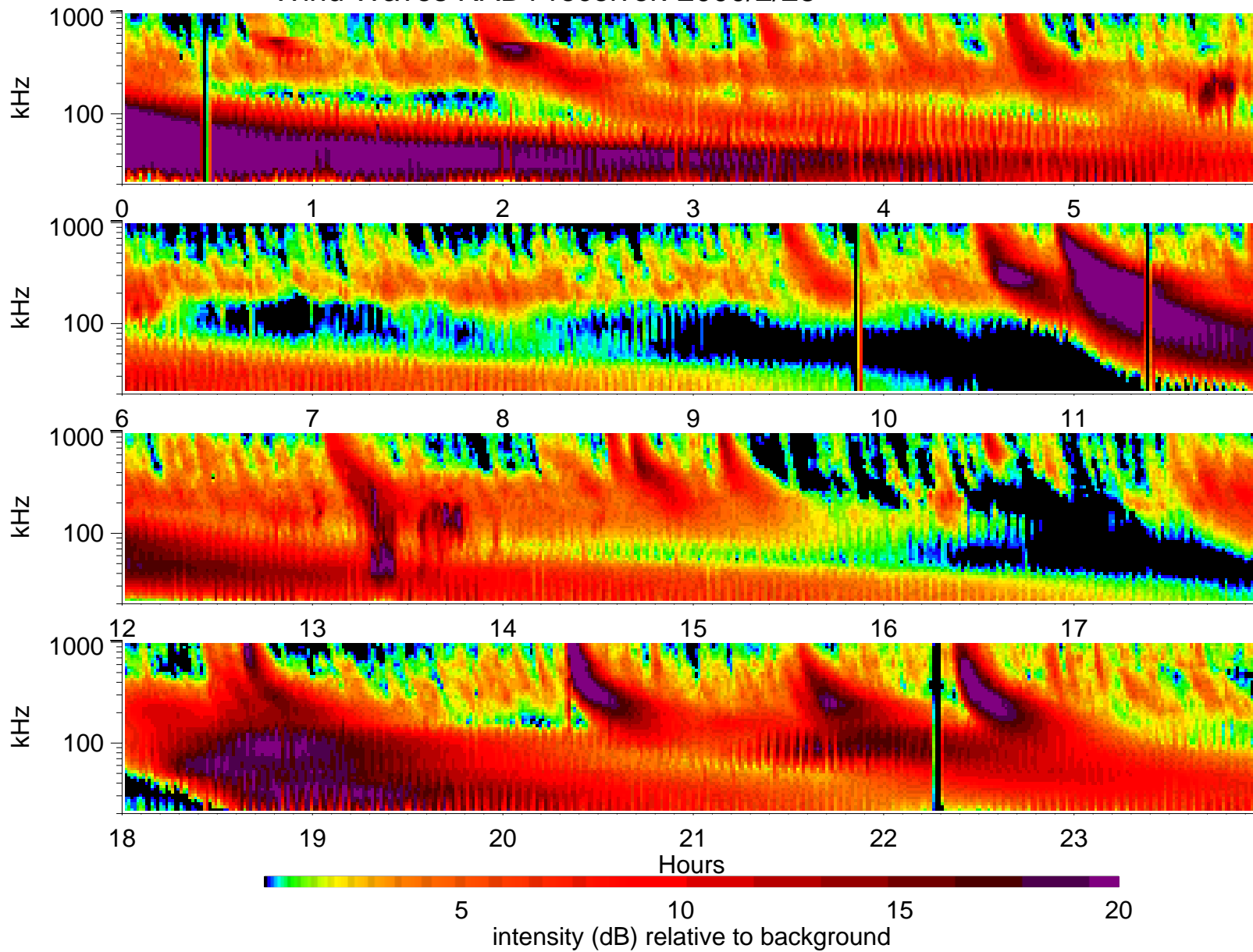
Wind Waves RAD1 receiver: 2000/2/28
