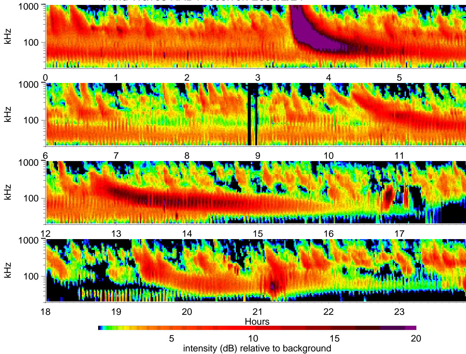
Wind Waves RAD1 receiver: 2000/2/24
