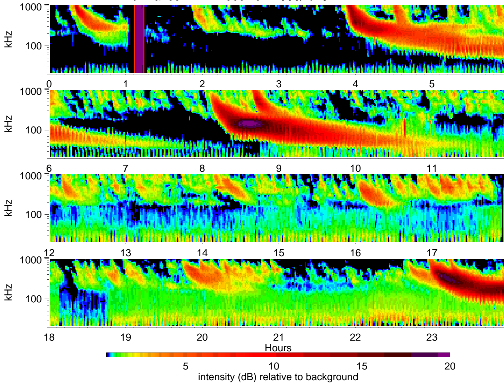
Wind Waves RAD1 receiver: 2000/2/19
