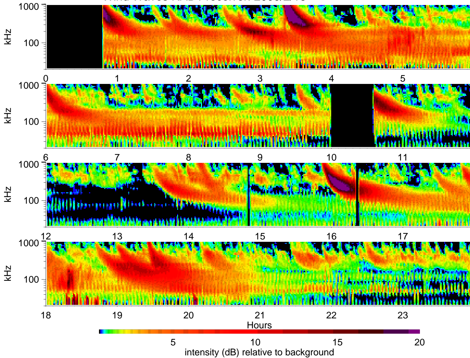
Wind Waves RAD1 receiver: 2000/2/16
