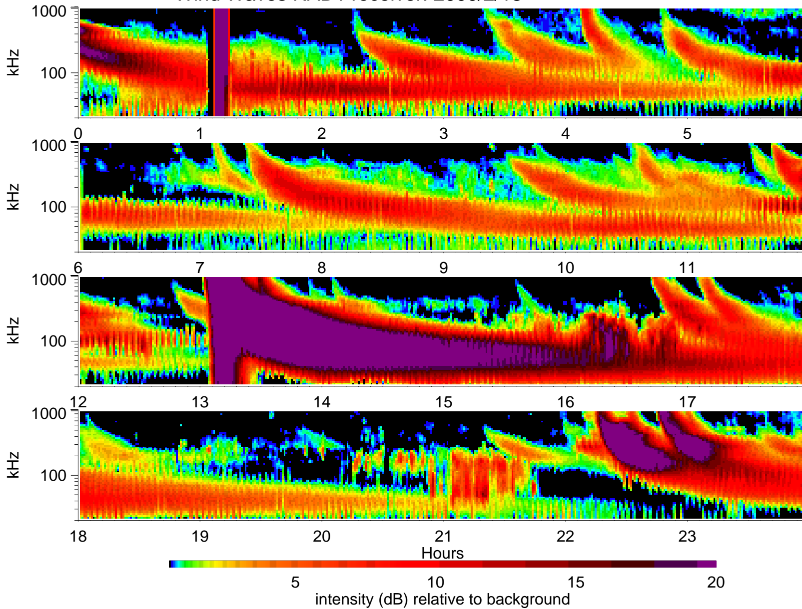
Wind Waves RAD1 receiver: 2000/2/13
