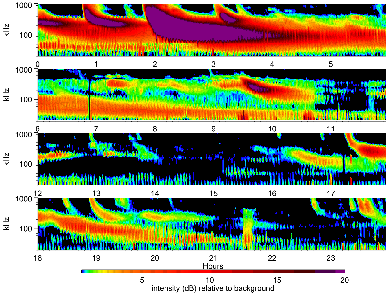
Wind Waves RAD1 receiver: 2000/2/10
