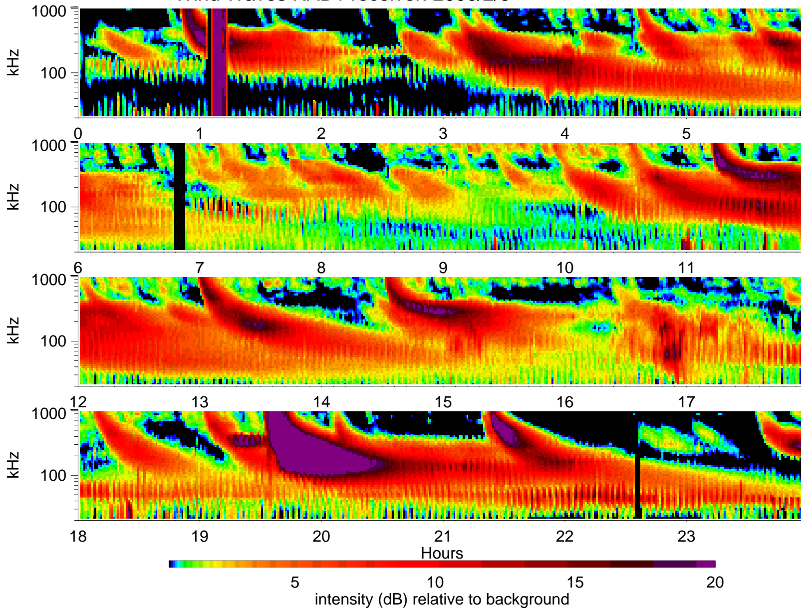
Wind Waves RAD1 receiver: 2000/2/9
