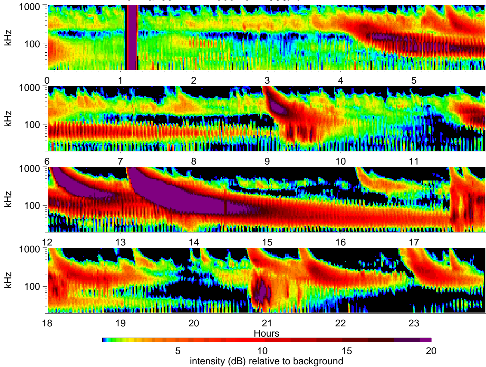
Wind Waves RAD1 receiver: 2000/2/7
