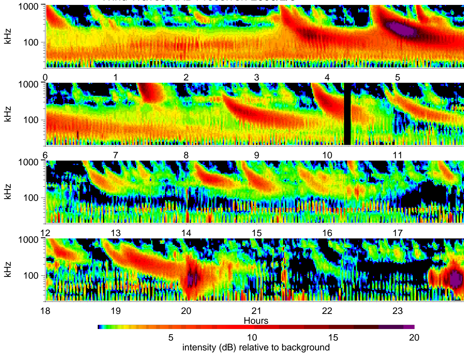
Wind Waves RAD1 receiver: 2000/2/6
