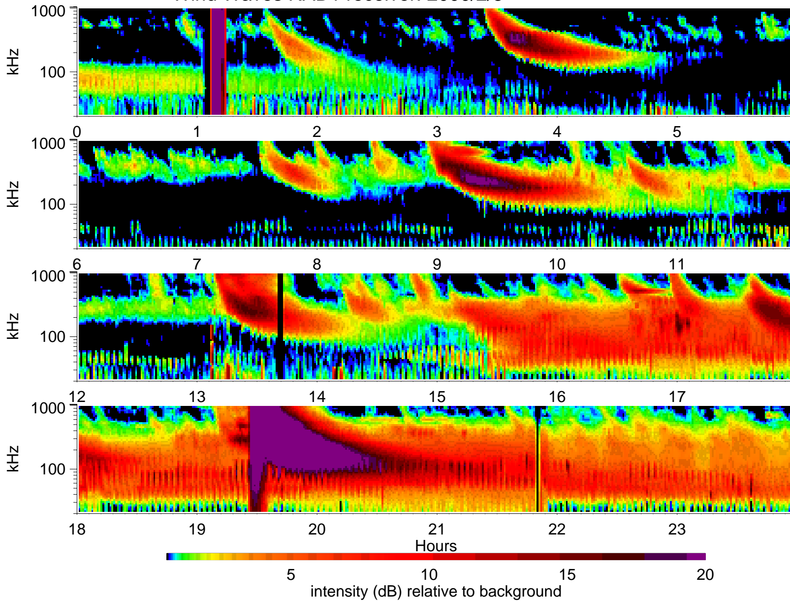
Wind Waves RAD1 receiver: 2000/2/5
