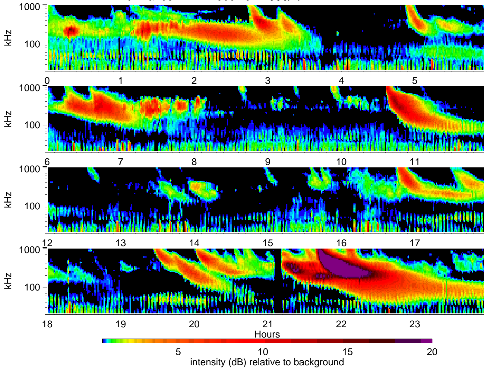
Wind Waves RAD1 receiver: 2000/2/4
