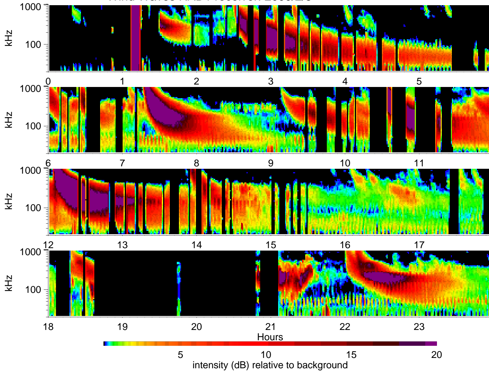
Wind Waves RAD1 receiver: 2000/2/3
