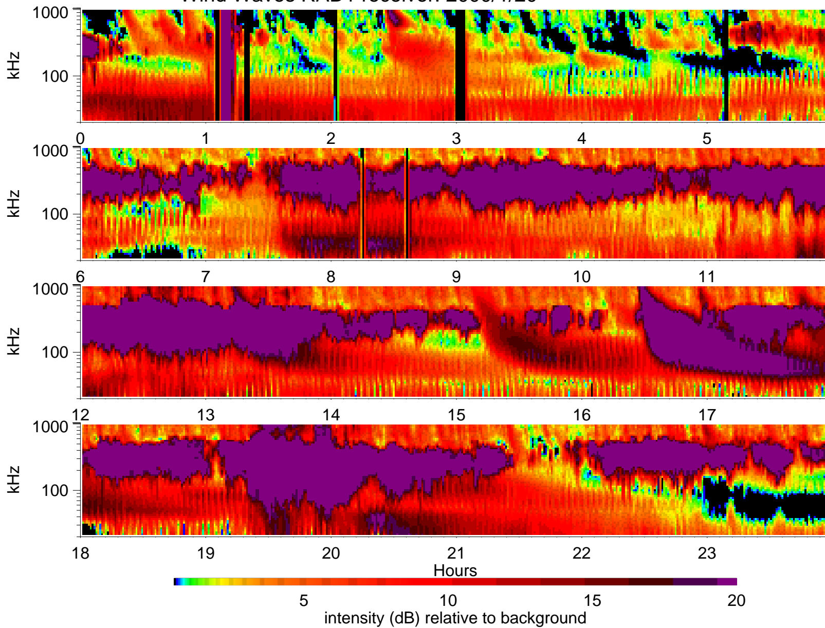
Wind Waves RAD1 receiver: 2000/1/20
