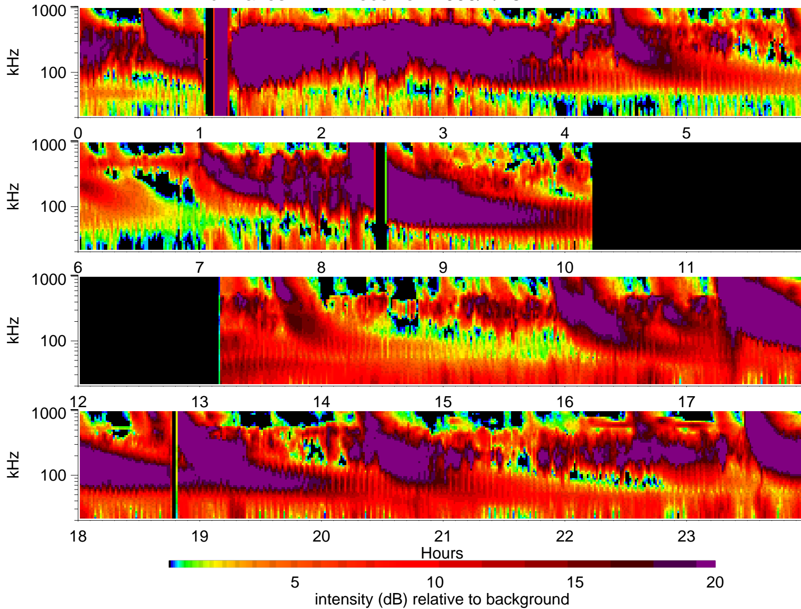
Wind Waves RAD1 receiver: 2000/1/18
