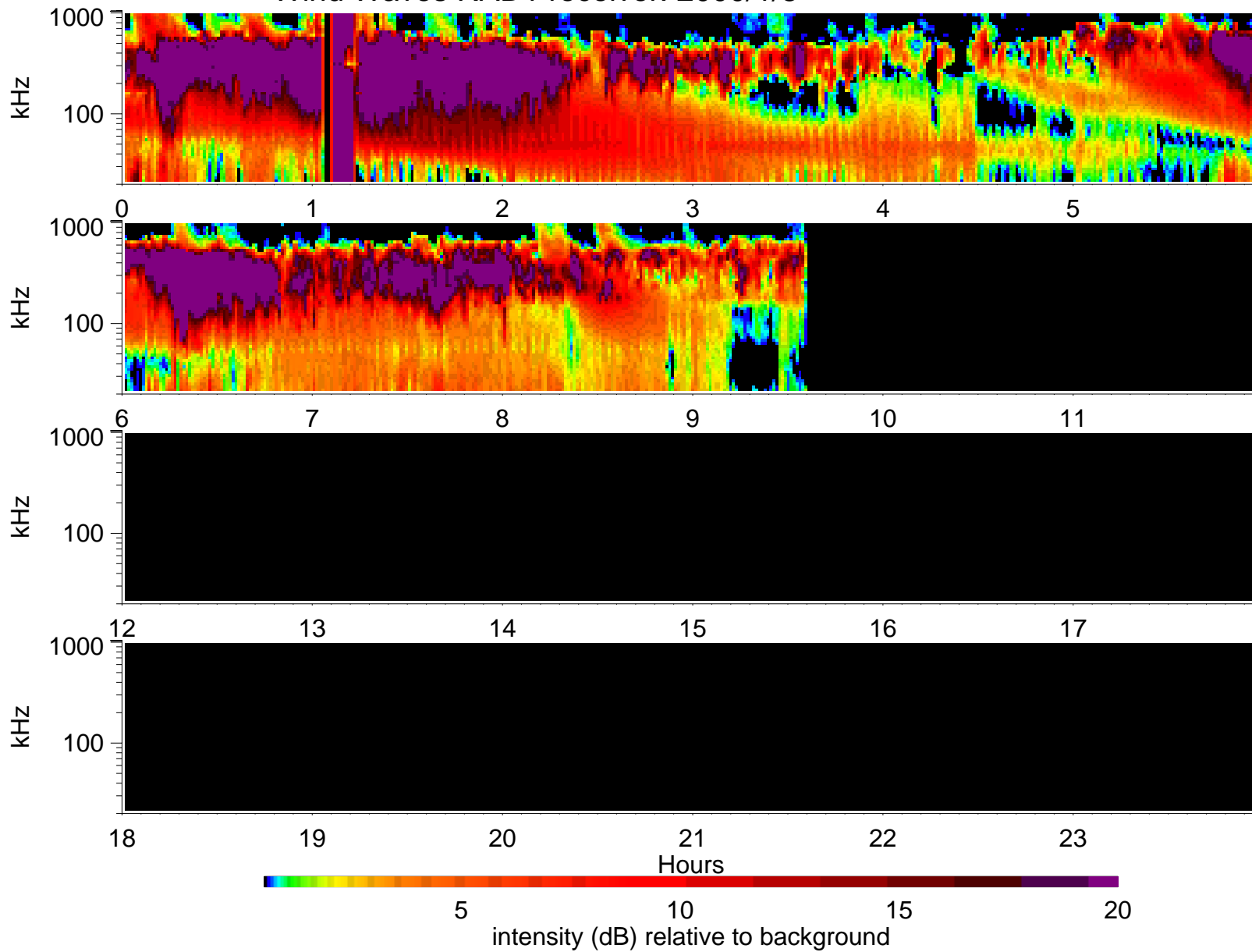
Wind Waves RAD1 receiver: 2000/1/8
