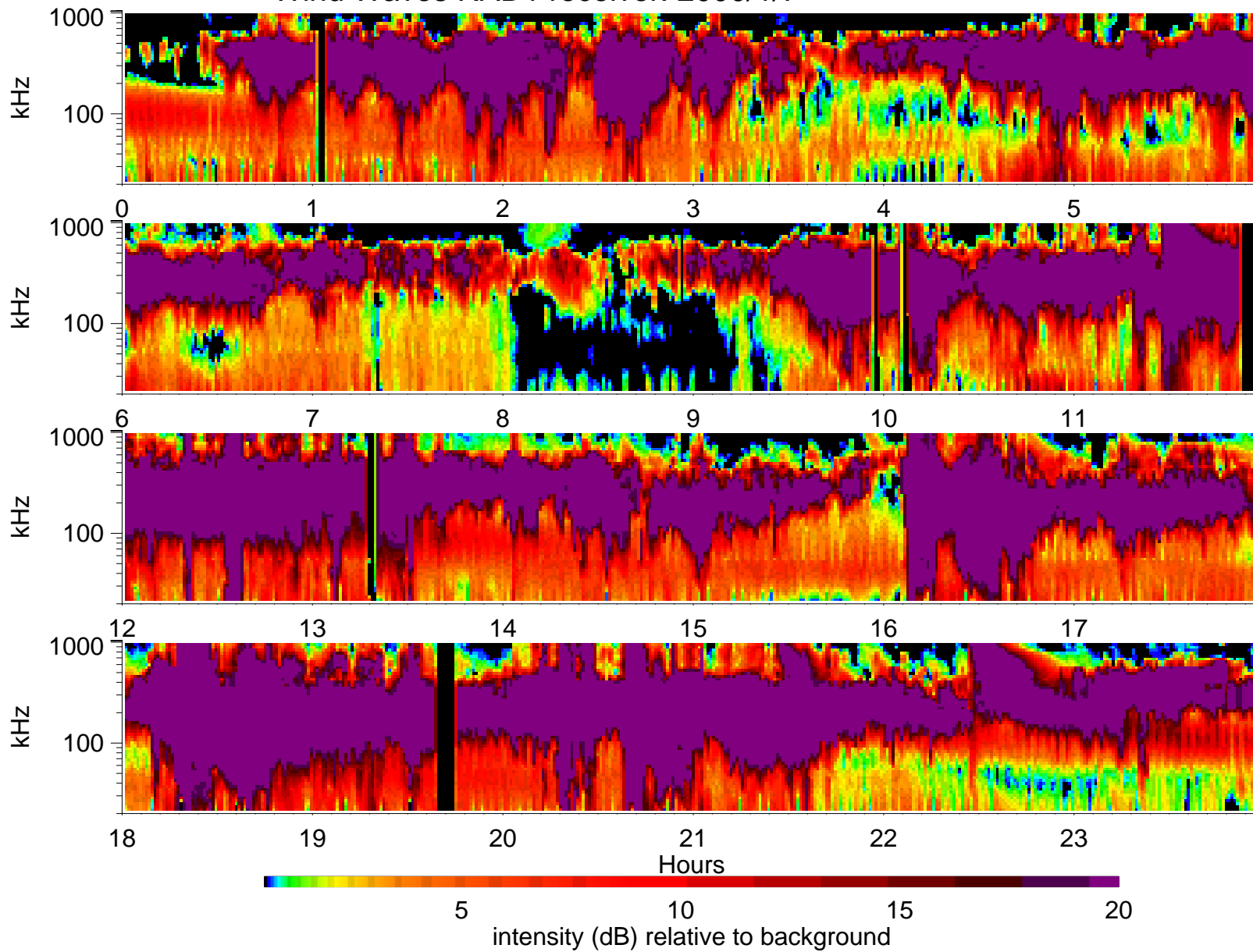
Wind Waves RAD1 receiver: 2000/1/7
