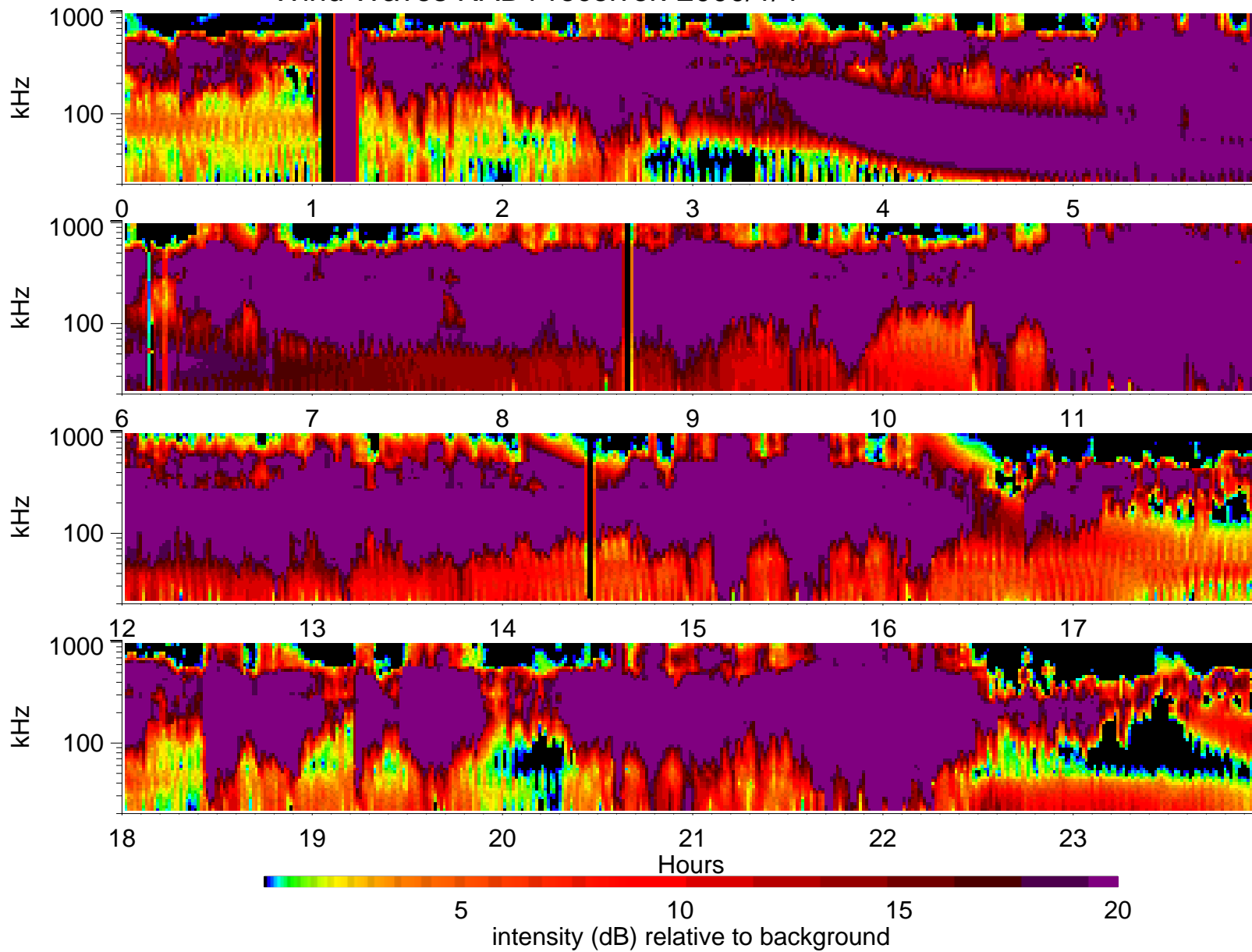
Wind Waves RAD1 receiver: 2000/1/4
