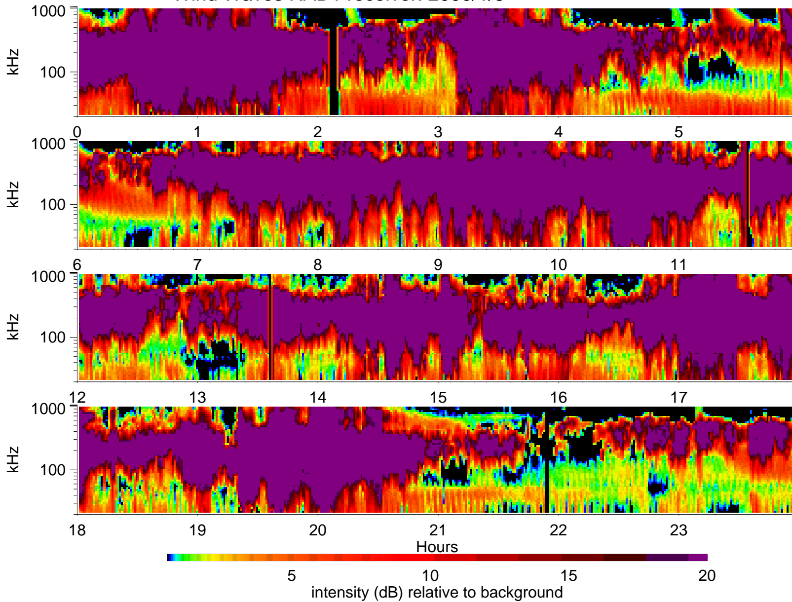
Wind Waves RAD1 receiver: 2000/1/3
