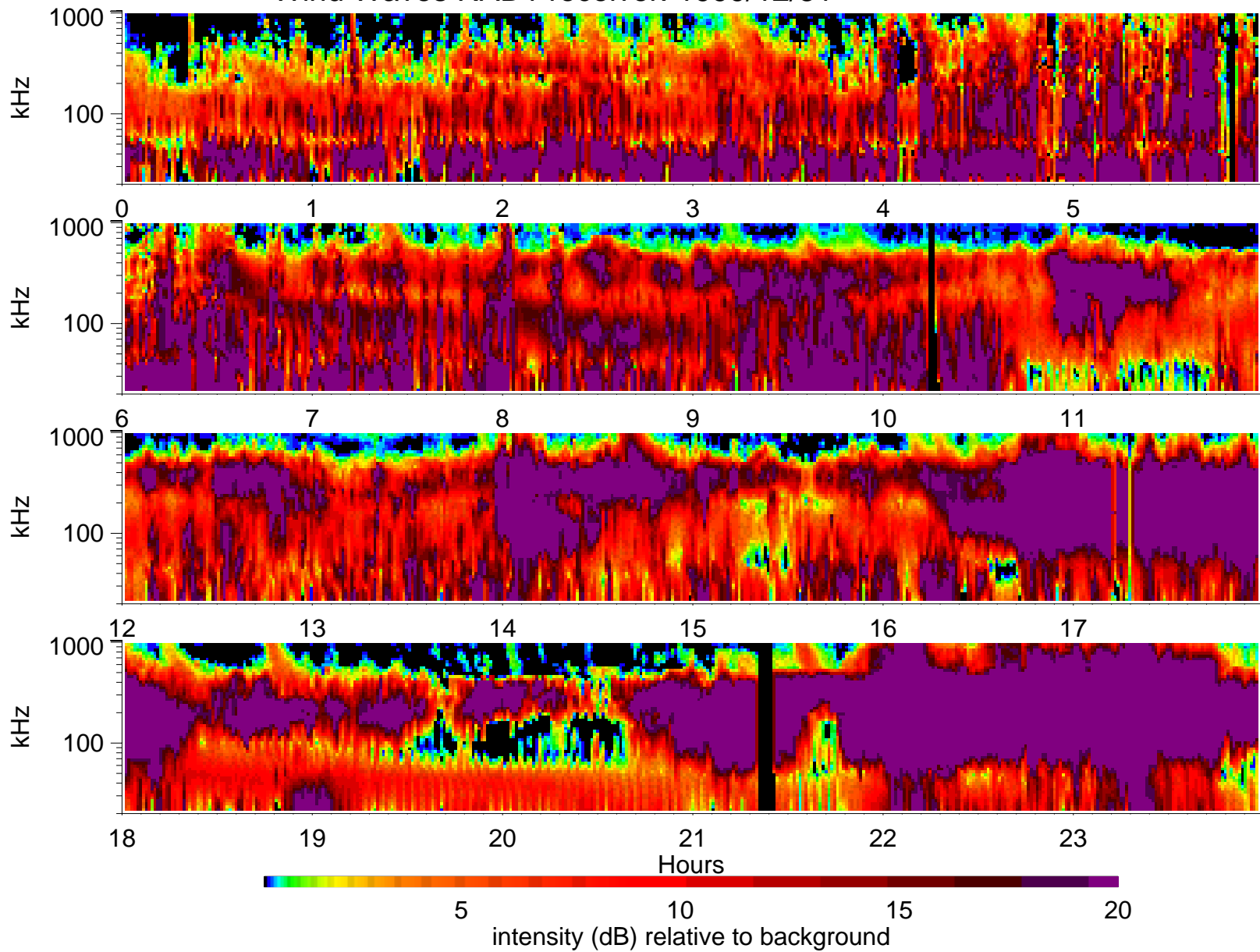
Wind Waves RAD1 receiver: 1999/12/31
