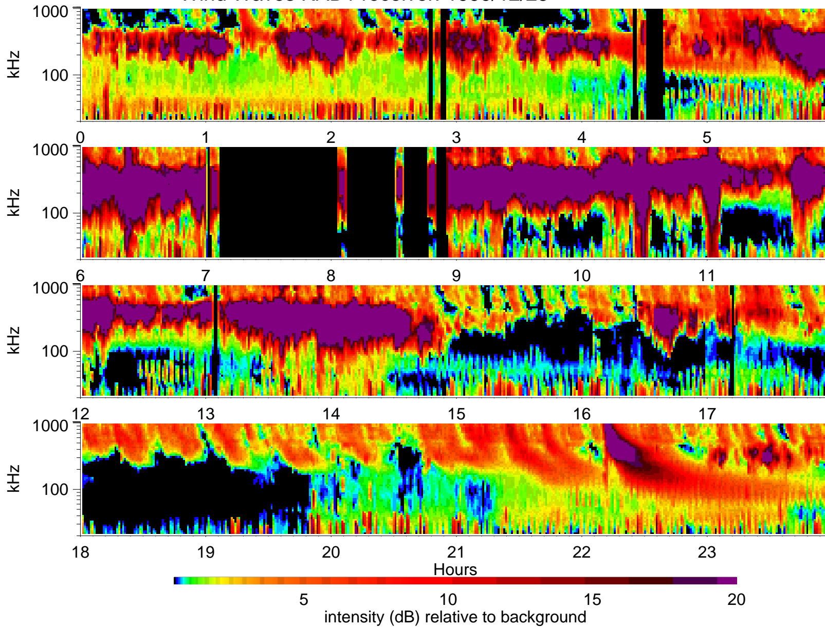
Wind Waves RAD1 receiver: 1999/12/25
