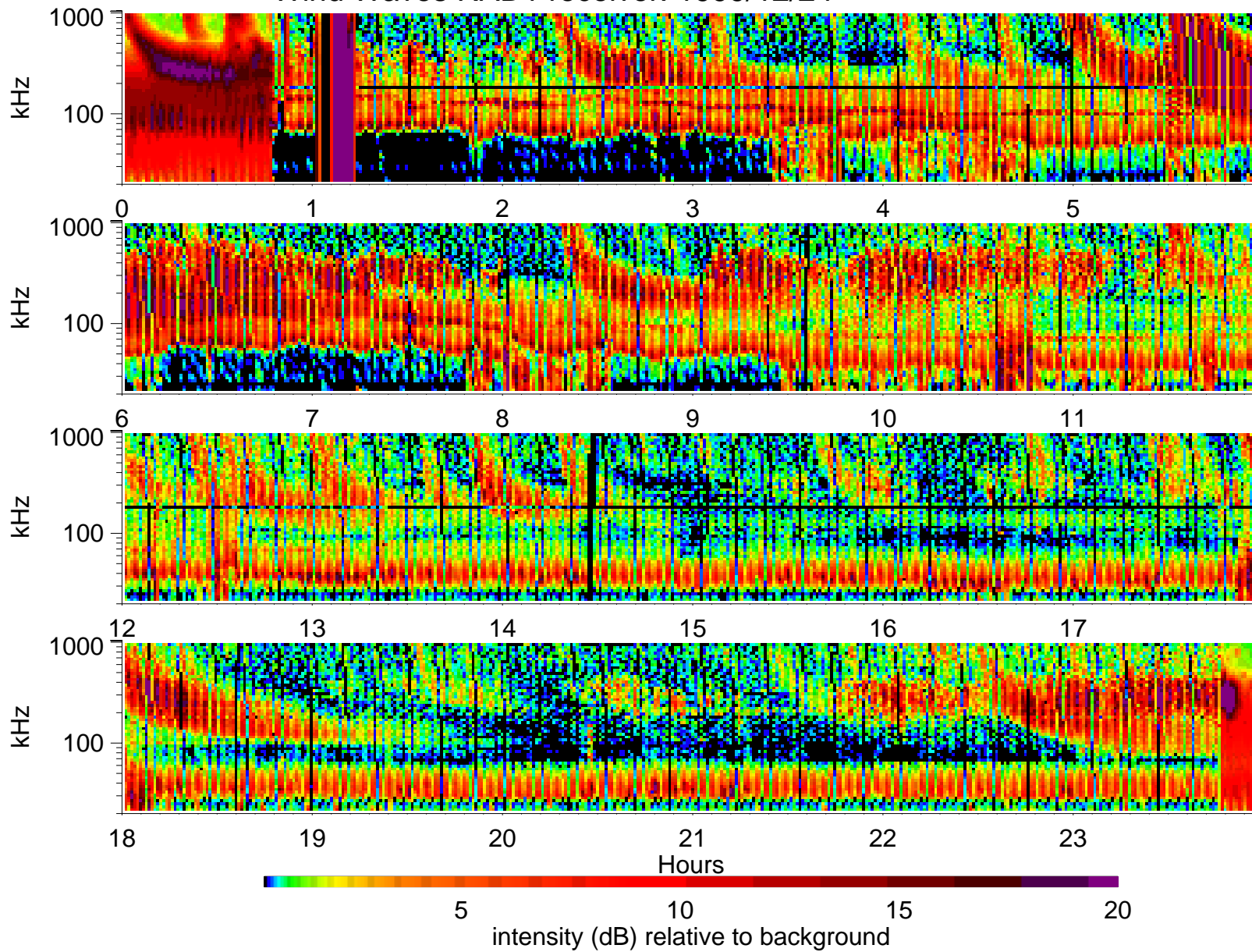
Wind Waves RAD1 receiver: 1999/12/24
