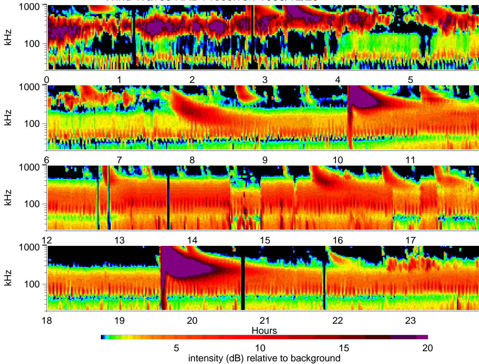
Wind Waves RAD1 receiver: 1999/12/23
