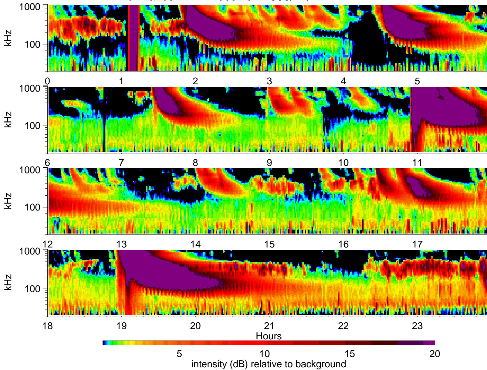
Wind Waves RAD1 receiver: 1999/12/22
