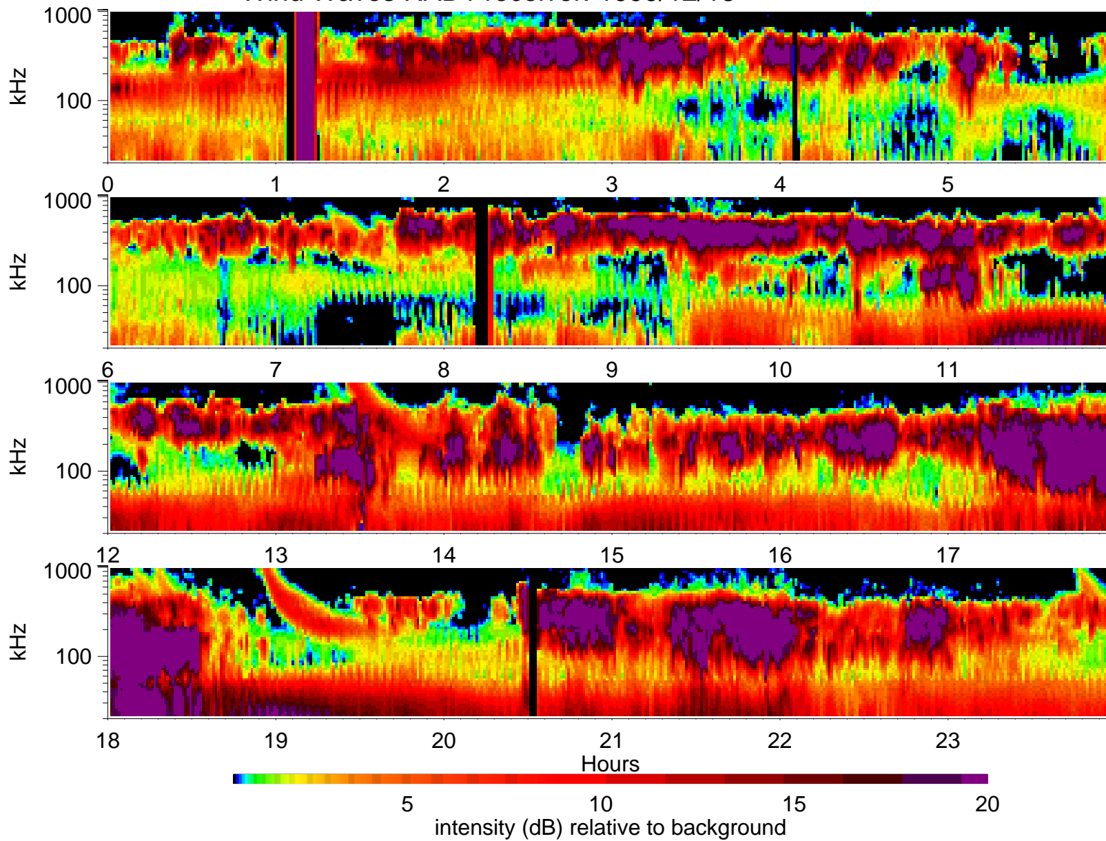
Wind Waves RAD1 receiver: 1999/12/18
