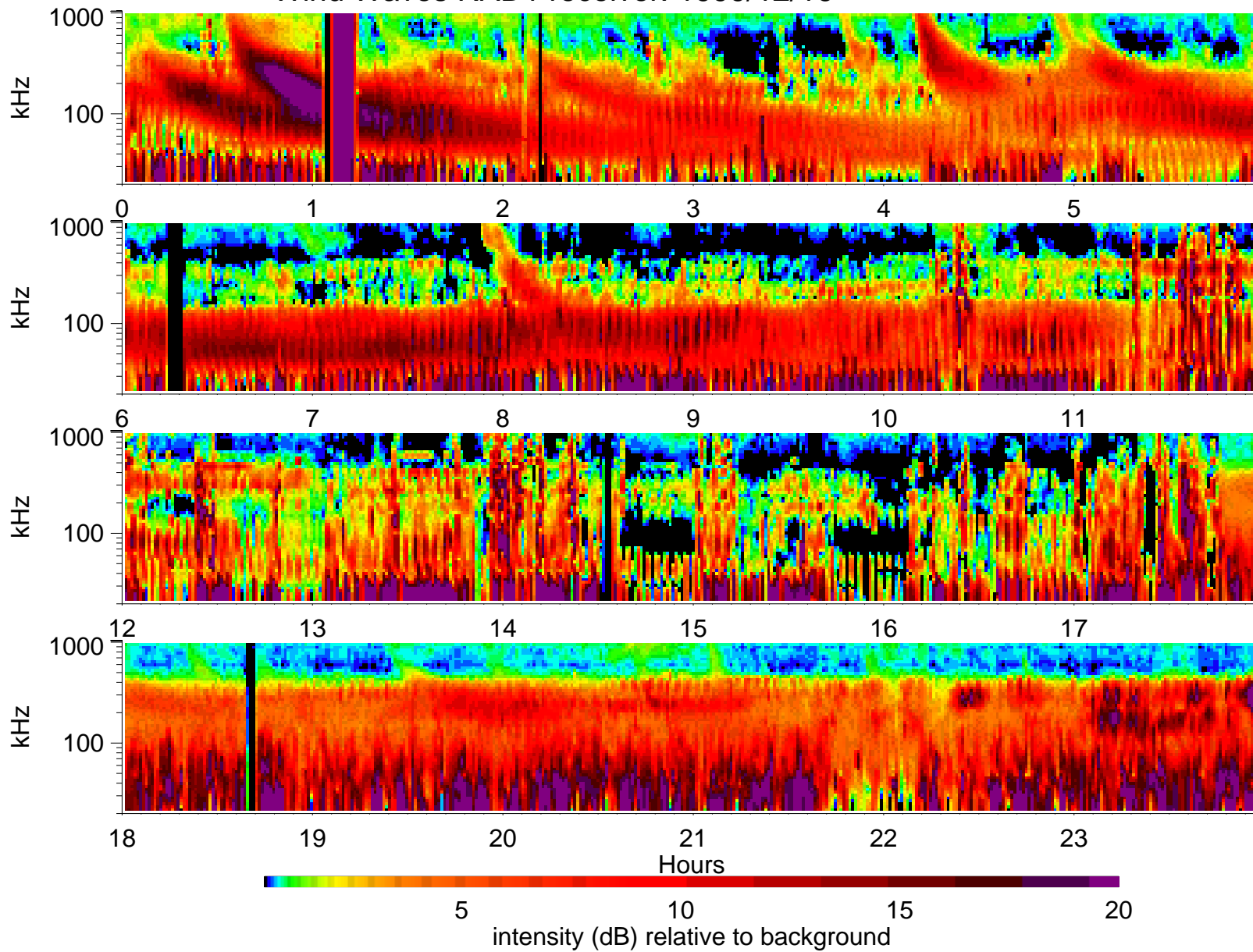
Wind Waves RAD1 receiver: 1999/12/16
