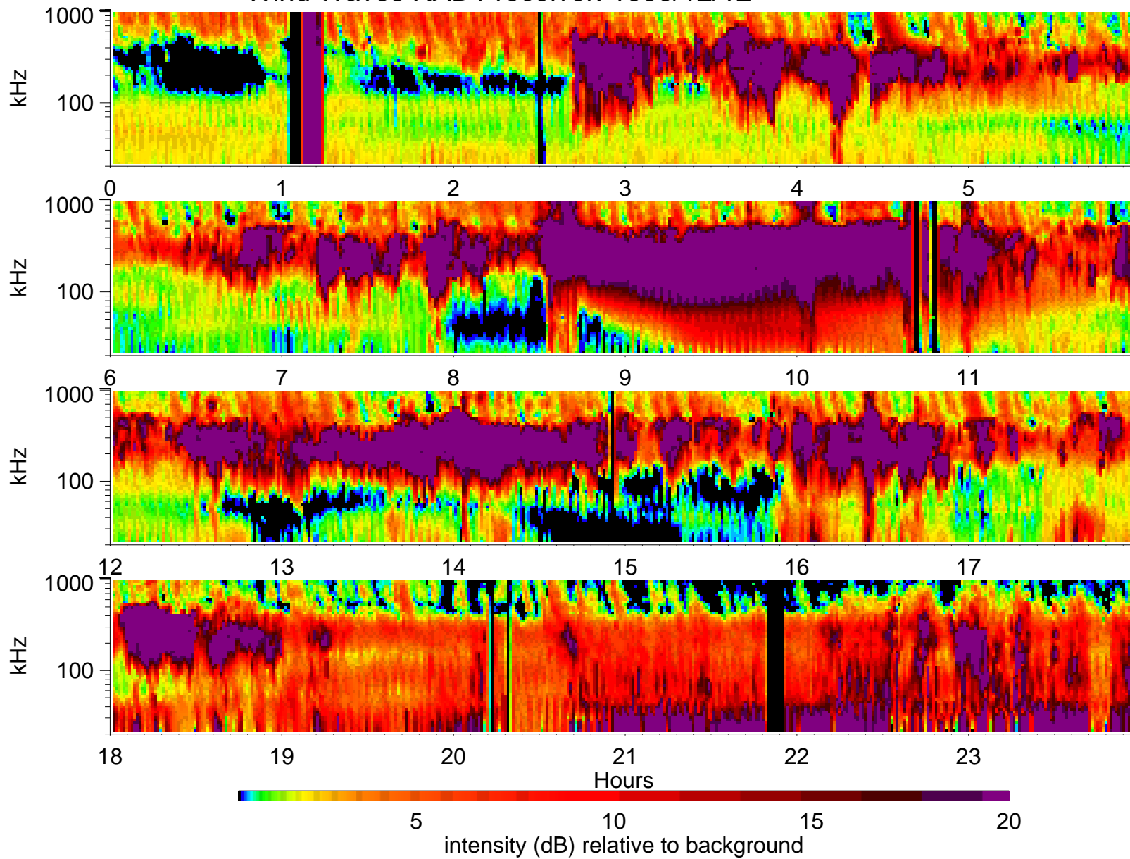
Wind Waves RAD1 receiver: 1999/12/12
