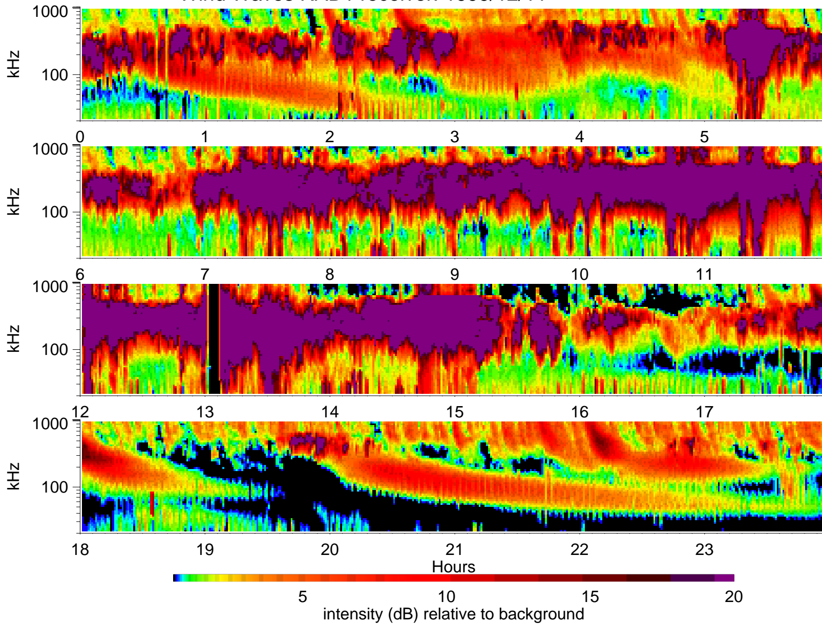
Wind Waves RAD1 receiver: 1999/12/11
