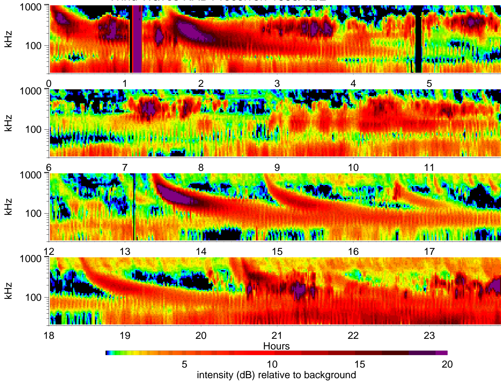
Wind Waves RAD1 receiver: 1999/12/2
