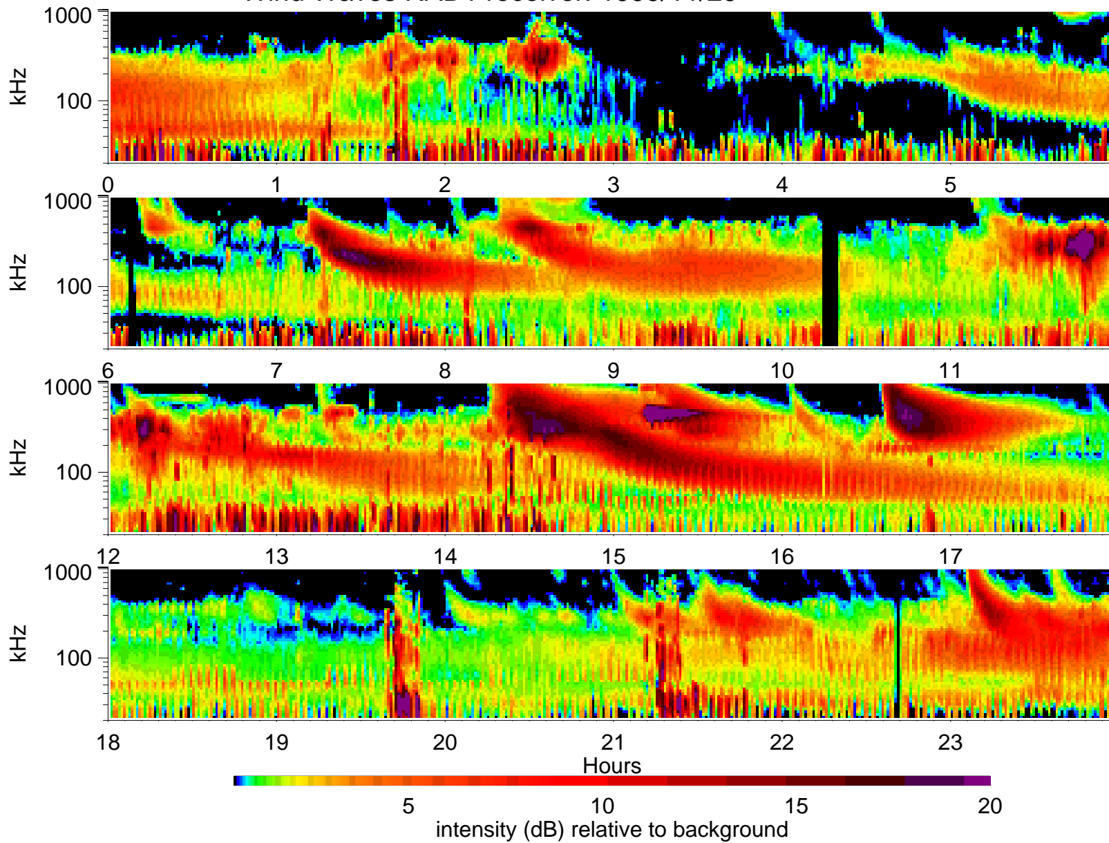
Wind Waves RAD1 receiver: 1999/11/29
