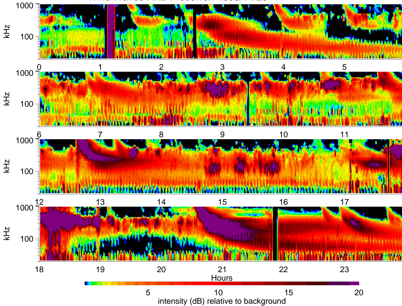
Wind Waves RAD1 receiver: 1999/11/28
