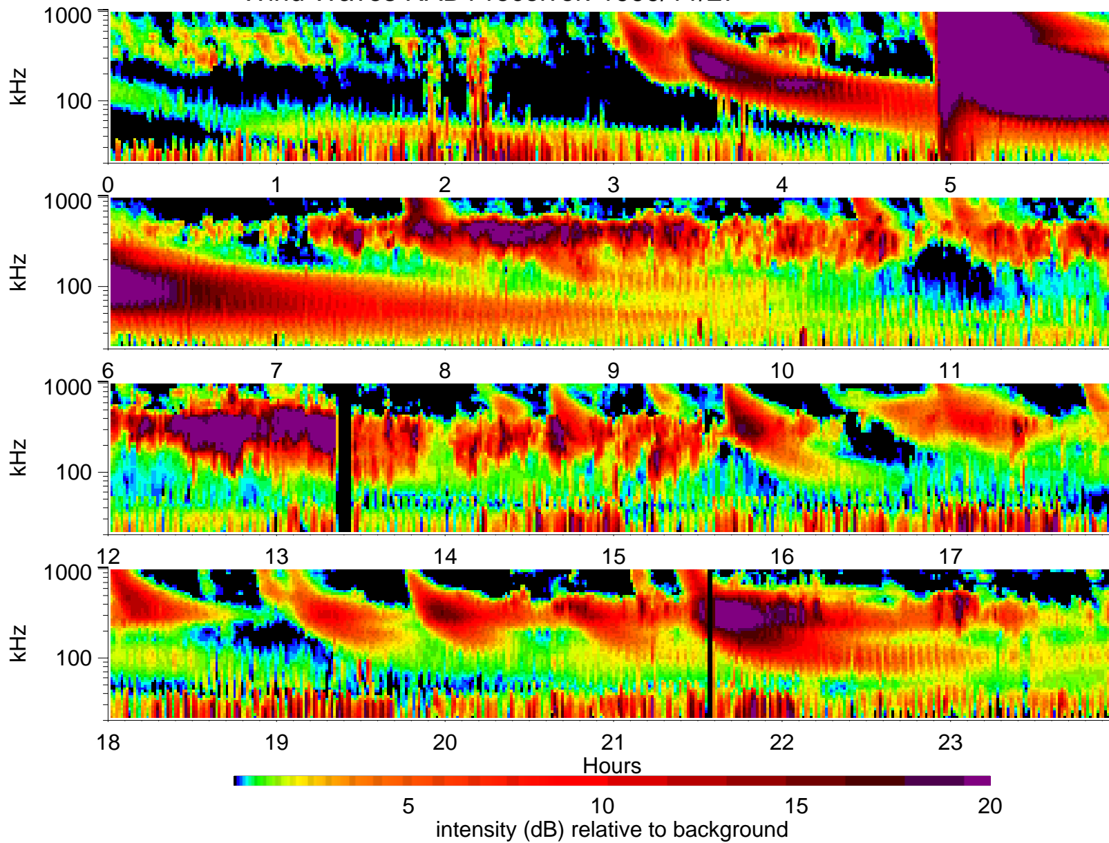
Wind Waves RAD1 receiver: 1999/11/27
