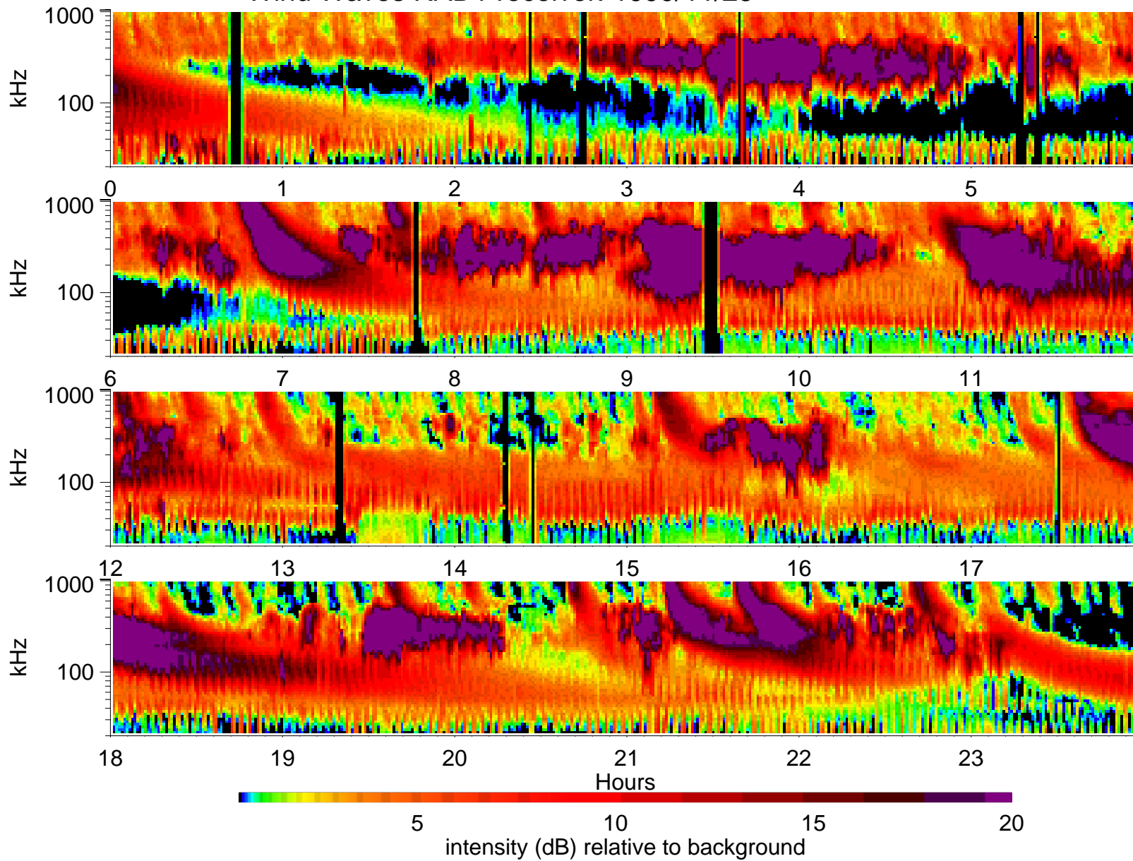
Wind Waves RAD1 receiver: 1999/11/25
