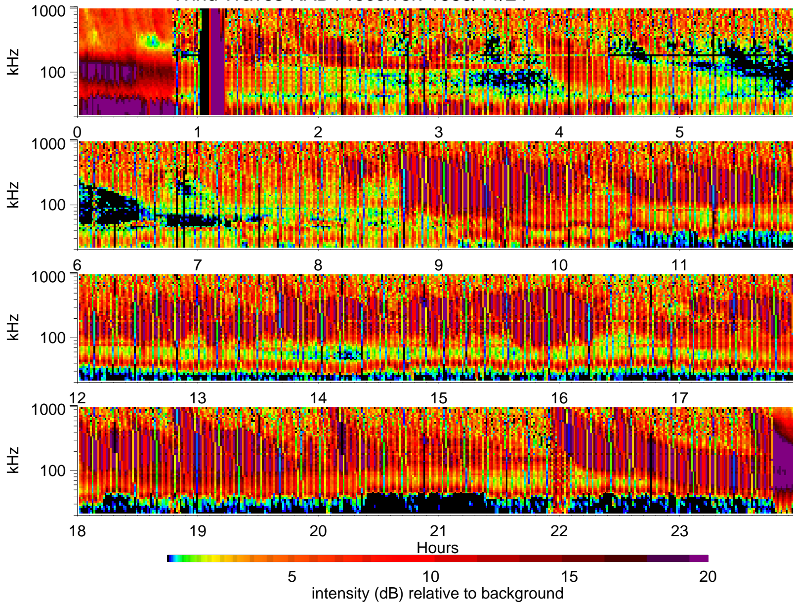
Wind Waves RAD1 receiver: 1999/11/24
