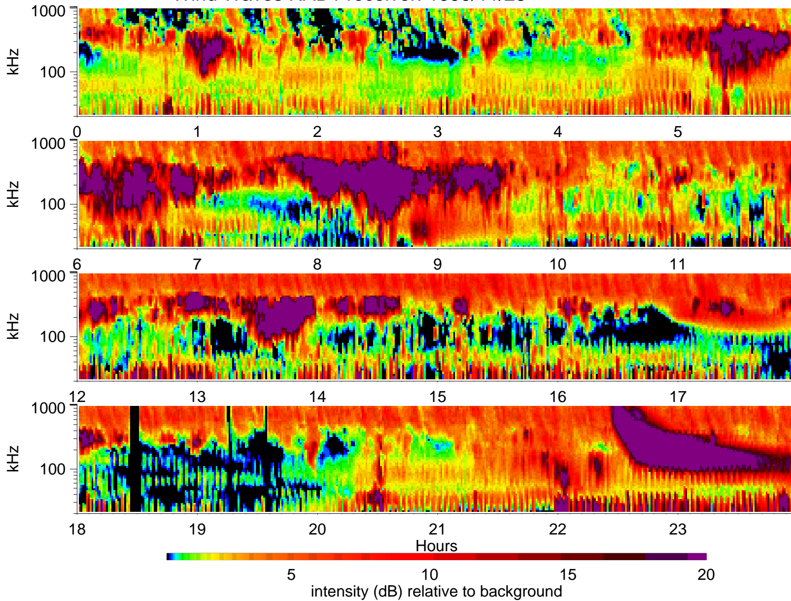
Wind Waves RAD1 receiver: 1999/11/23
