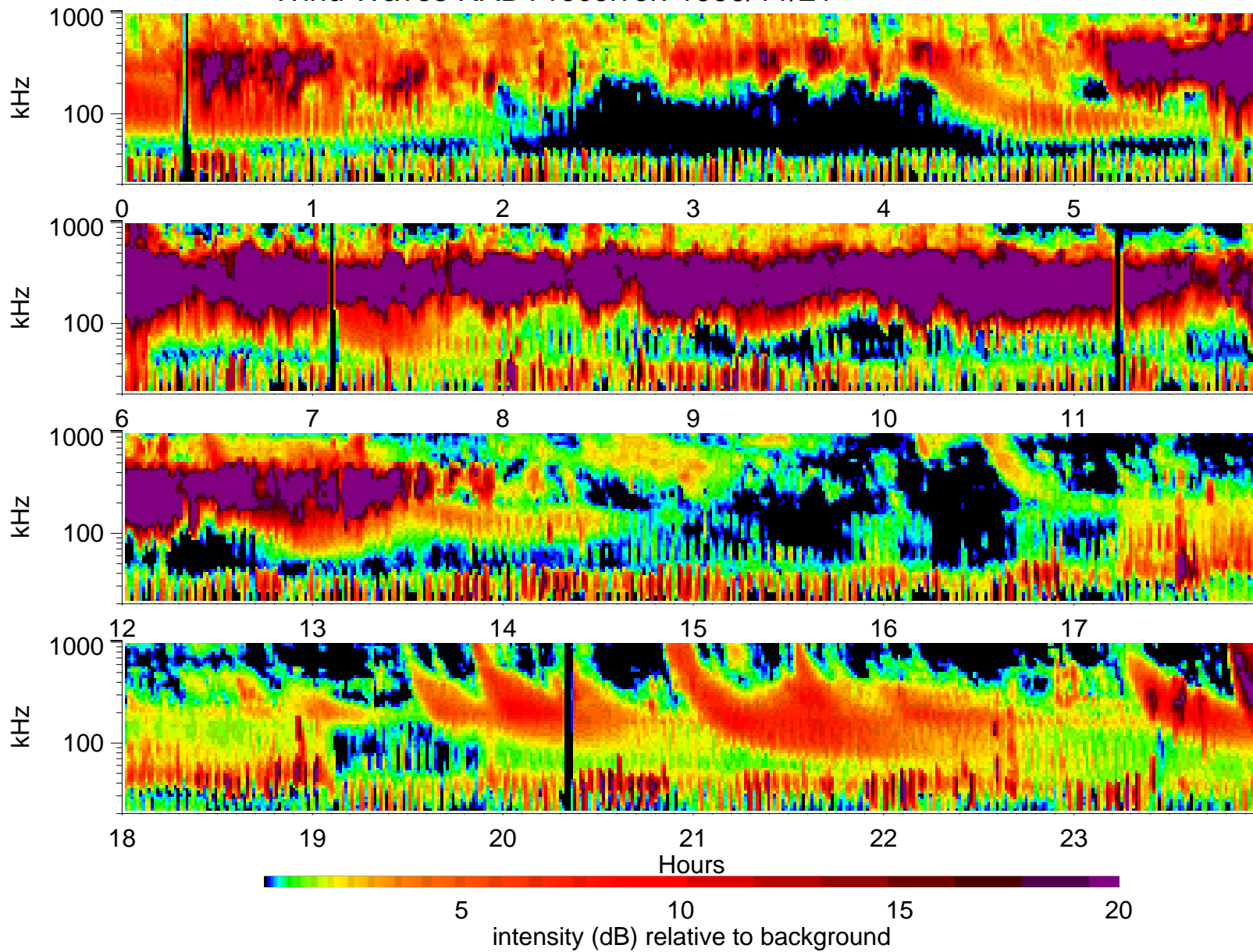
Wind Waves RAD1 receiver: 1999/11/21
