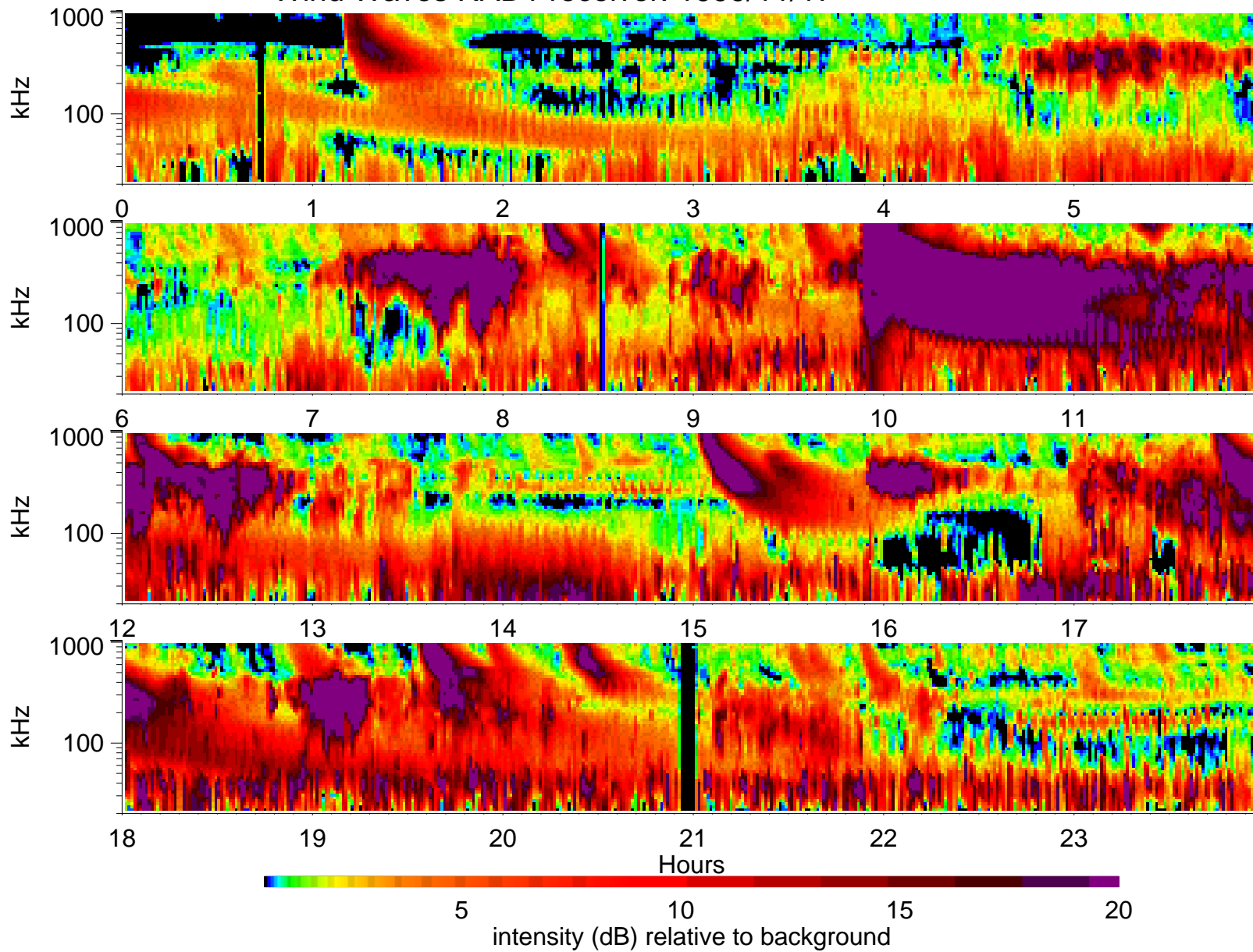
Wind Waves RAD1 receiver: 1999/11/17
