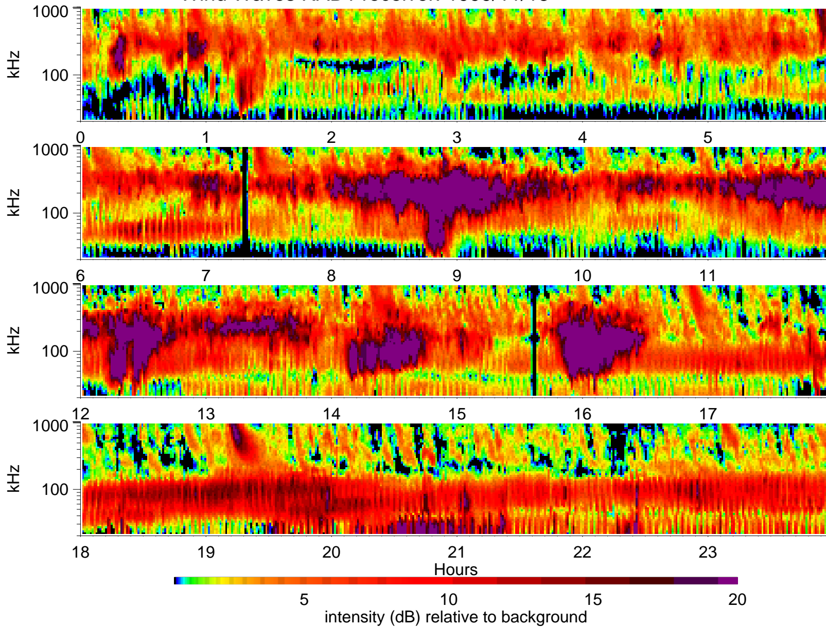
Wind Waves RAD1 receiver: 1999/11/13
