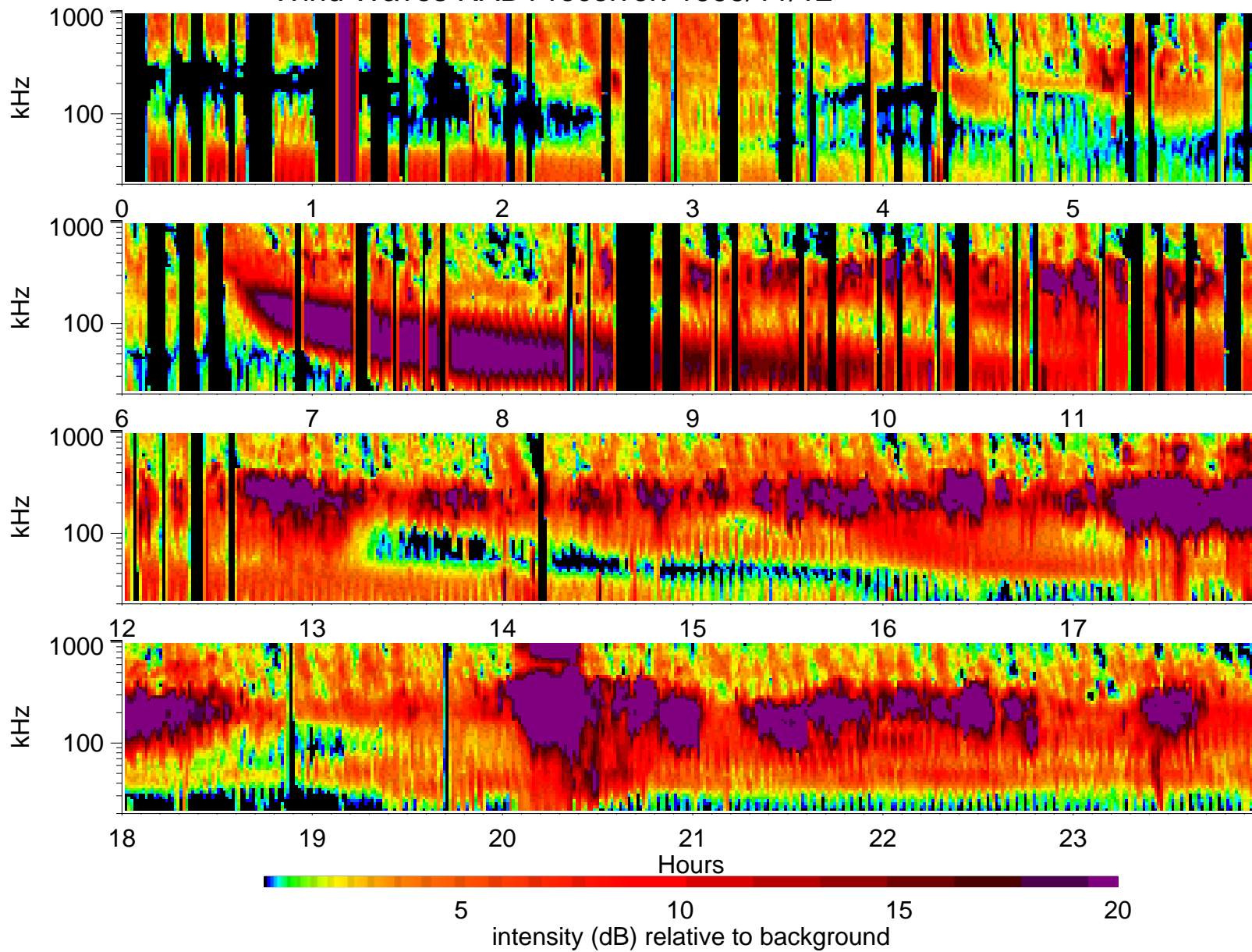
Wind Waves RAD1 receiver: 1999/11/12
