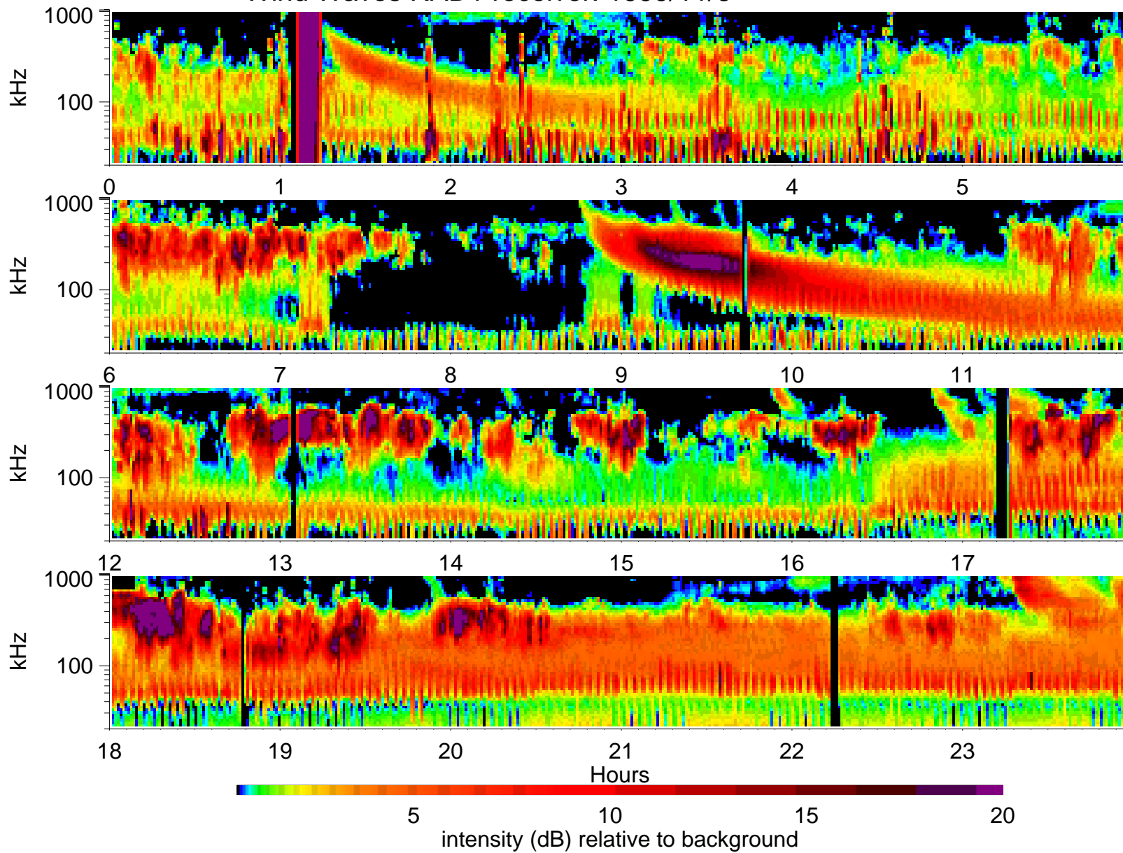
Wind Waves RAD1 receiver: 1999/11/6
