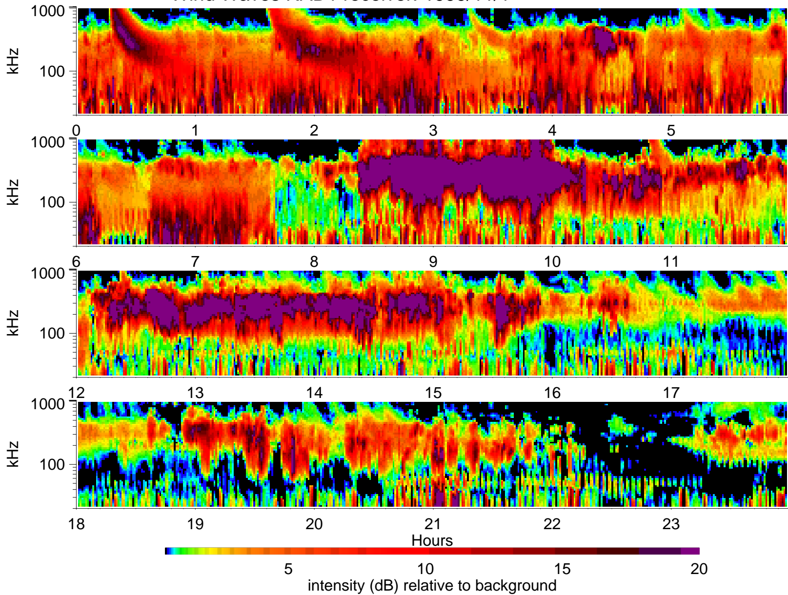
Wind Waves RAD1 receiver: 1999/11/1
