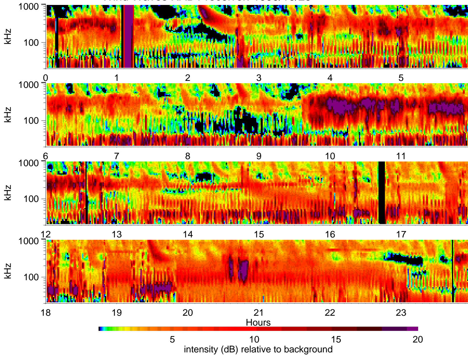
Wind Waves RAD1 receiver: 1999/10/29
