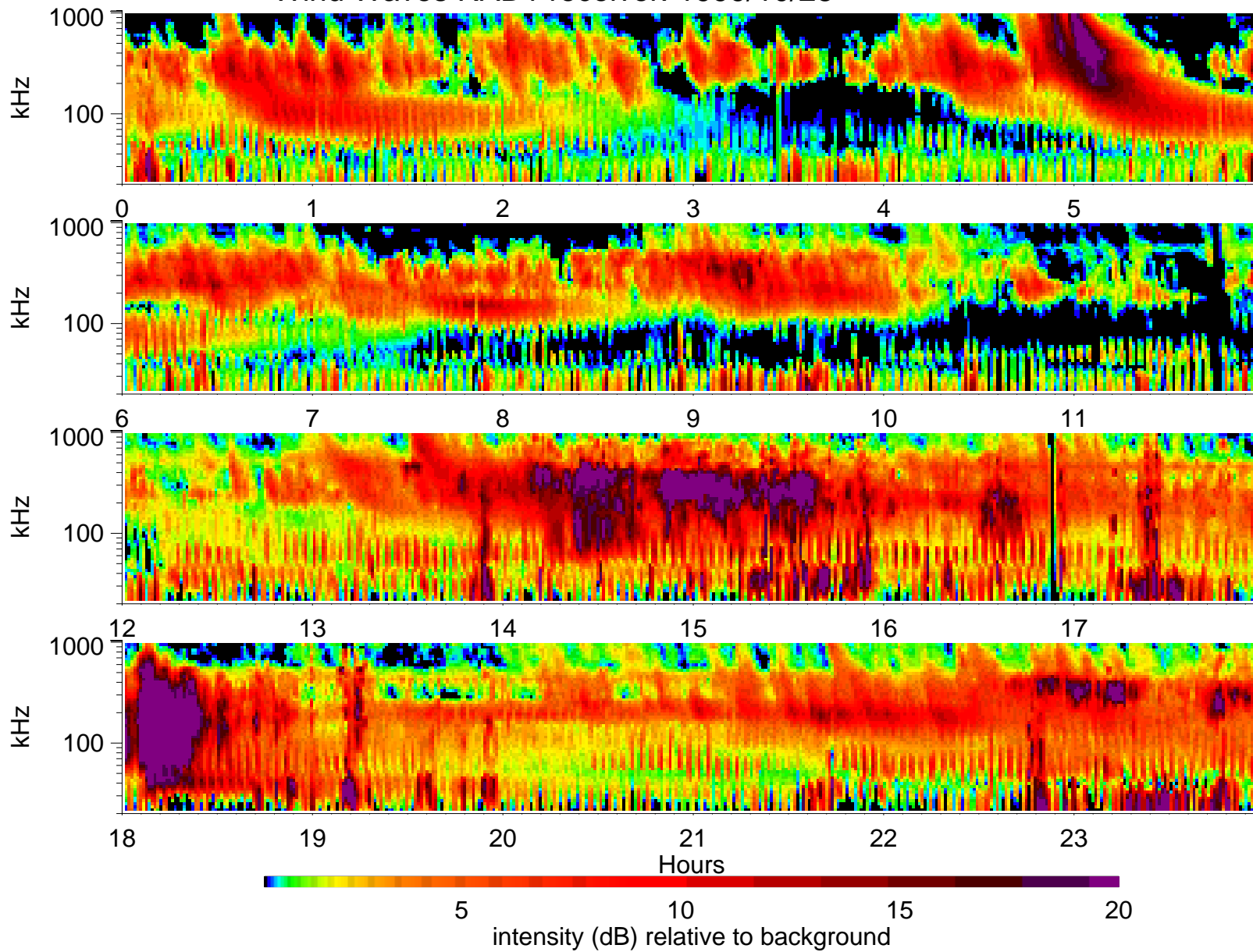
Wind Waves RAD1 receiver: 1999/10/28
