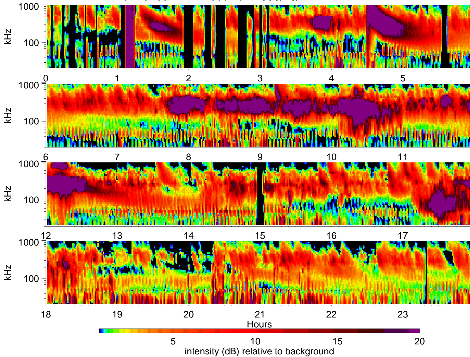
Wind Waves RAD1 receiver: 1999/10/27
