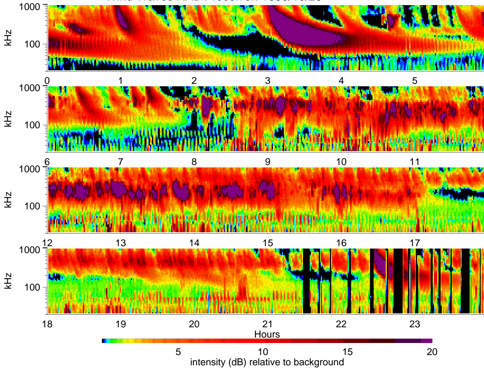
Wind Waves RAD1 receiver: 1999/10/26
