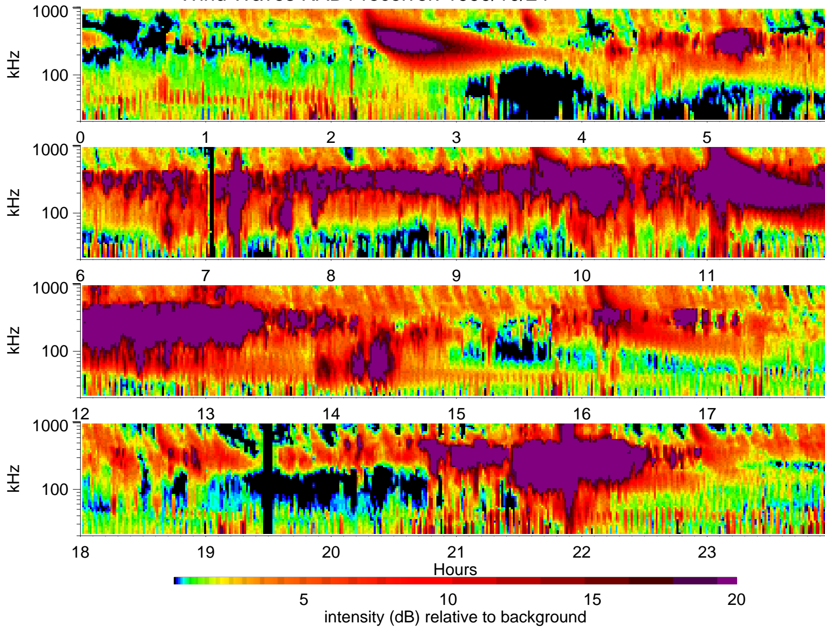
Wind Waves RAD1 receiver: 1999/10/24
