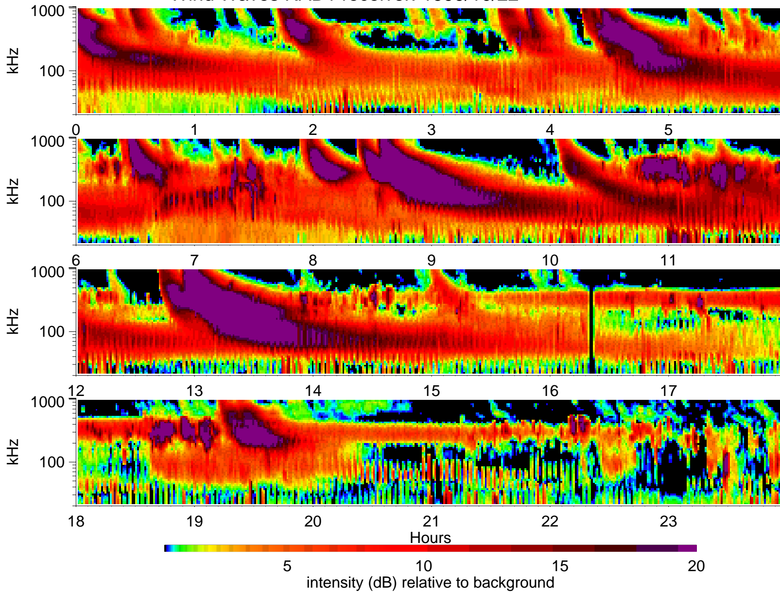
Wind Waves RAD1 receiver: 1999/10/22
