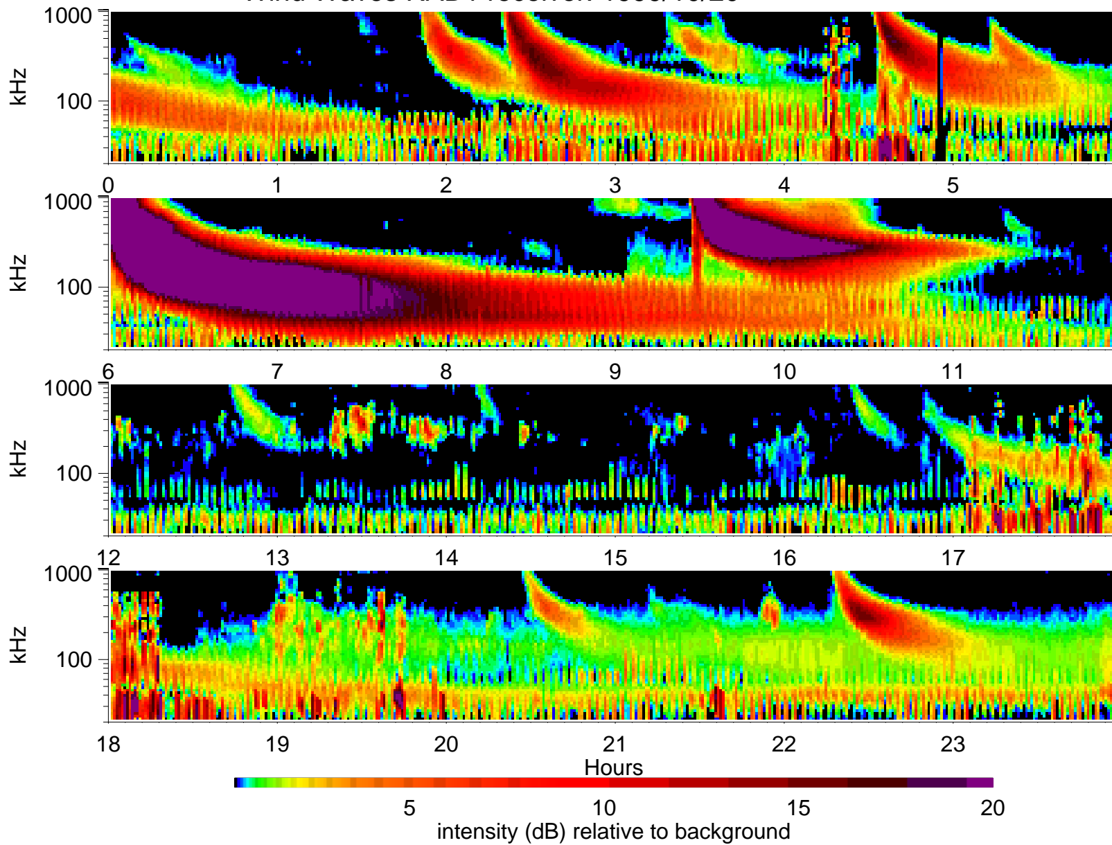
Wind Waves RAD1 receiver: 1999/10/20
