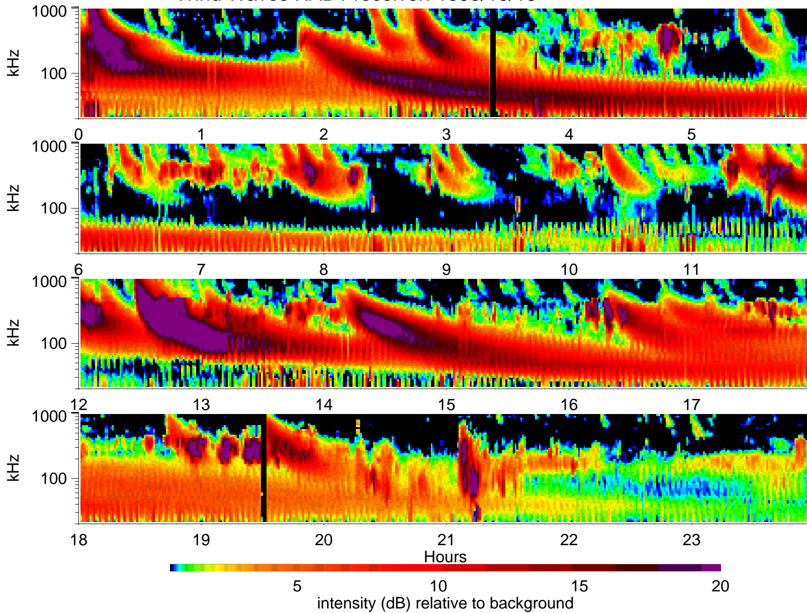
Wind Waves RAD1 receiver: 1999/10/18
